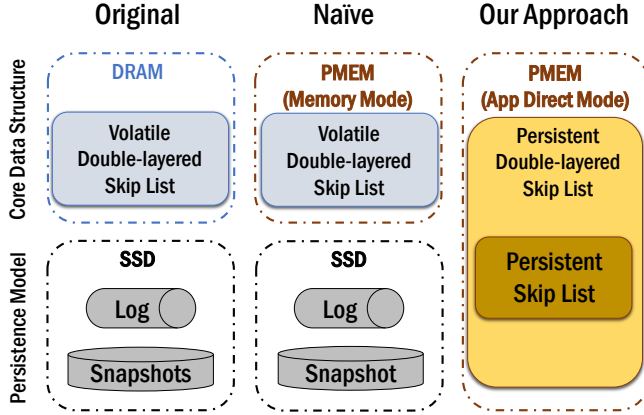
Figure 8: Different Ways of Using PMEM in FEDB
