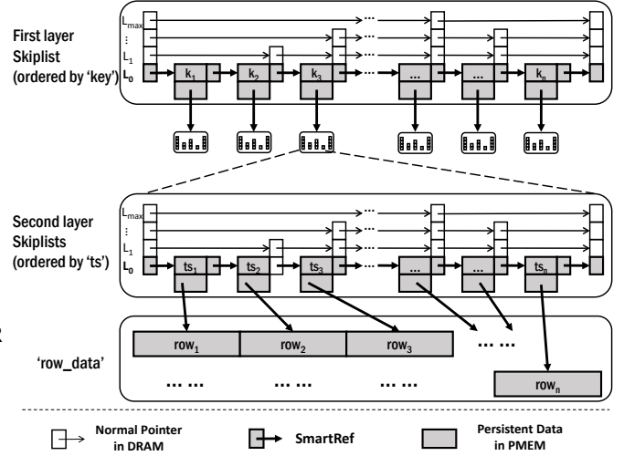
Figure 7: In-memory Double-layered (Persistent) Skiplist
