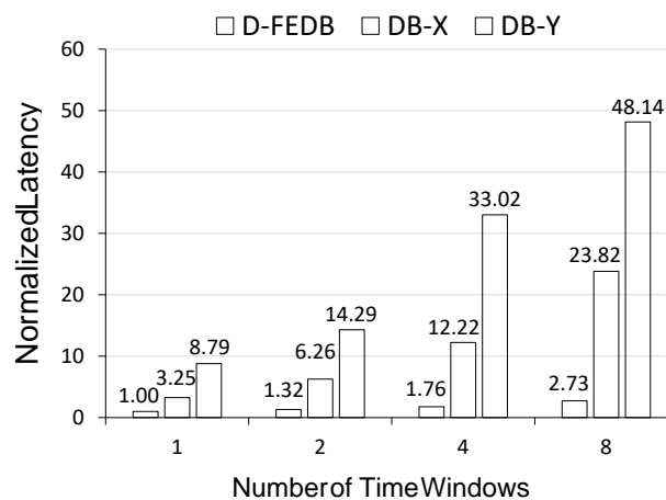
Figure 9: Latency Comparison of On-line Feature Extraction over Varied Number of Time Windows
