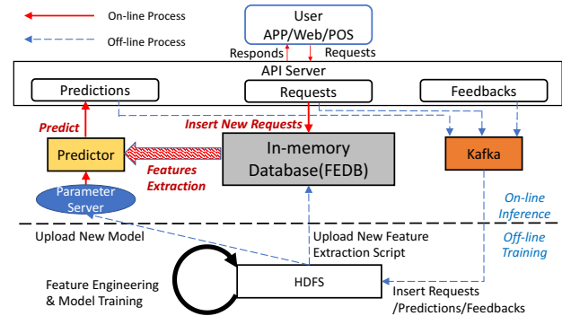
Figure 1: Workflow of AI-powered OLDA Systems
