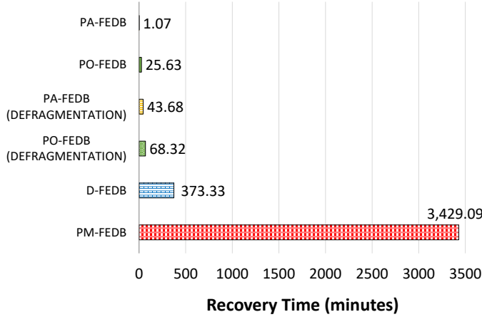
Figure 14: Recovery Time under Real-world Workloads
