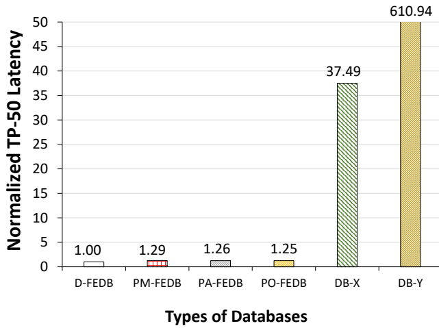
Figure 12: Latency under Real-world Workloads On Different DBMS
