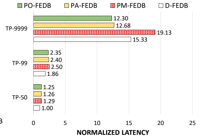
Figure 13: Tail Latency of Different FEDB’s Variants under Real-world Workloads
